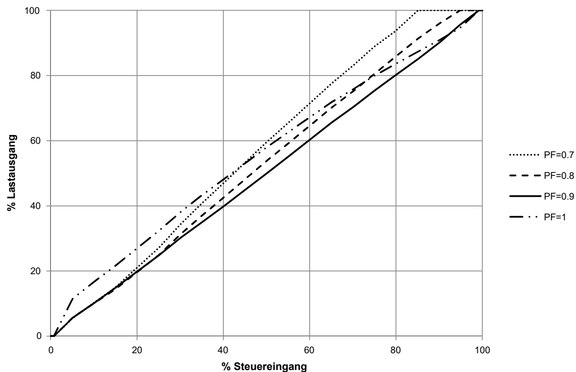
3-phasige 4-Leiter-Systeme
