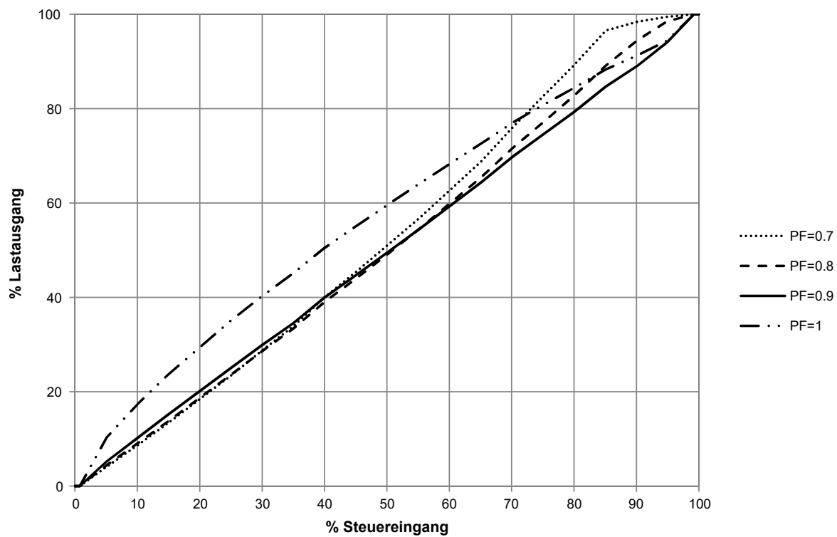
3-phasige 4-Leiter-Systeme
