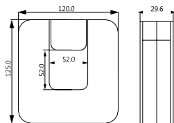
1000 A CT
