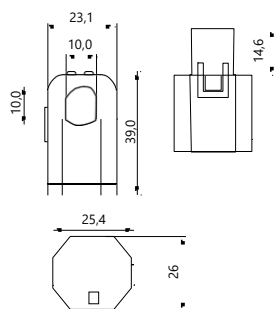
70 A CT
