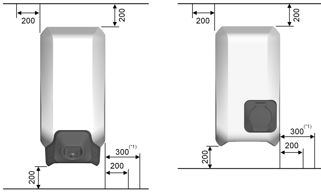
Fig. 8-2: Minimum distances in millimetres
