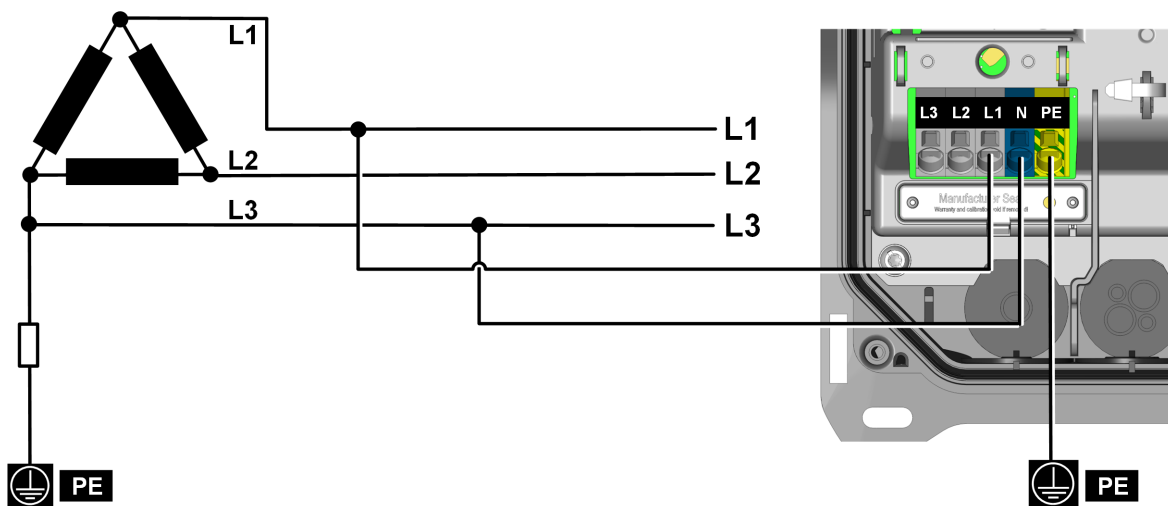
Fig. 9-5: Connection to a three-wire IT system with 230 V
