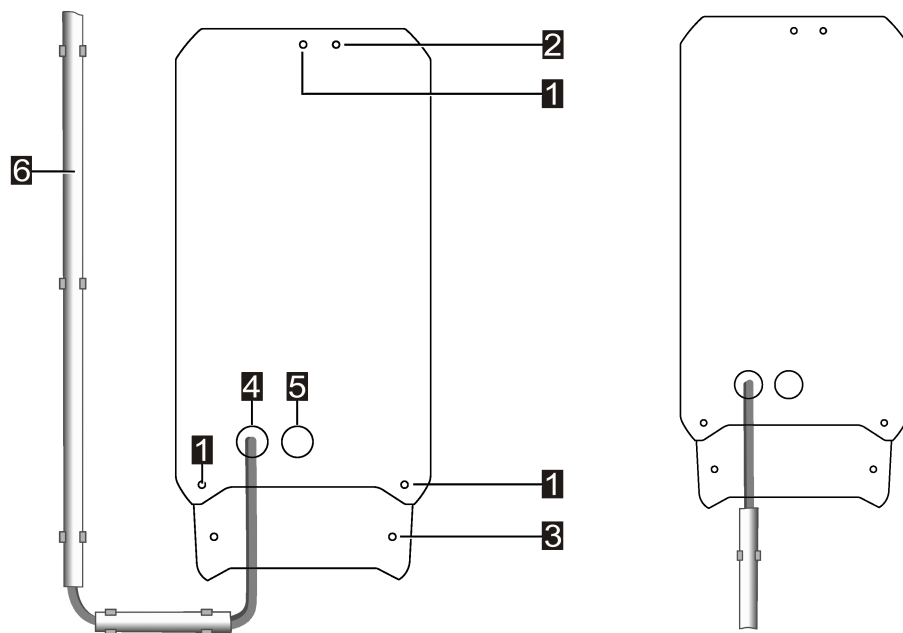
Fig. 8-3: Example: Mounting points and surface-mounted cable routing
