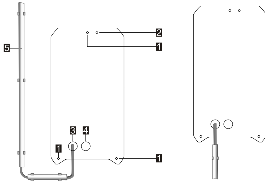
Fig. 8-4: Example: Mounting points and surface-mounted cable routing
