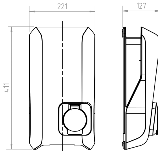
Dimensions in millimeter
