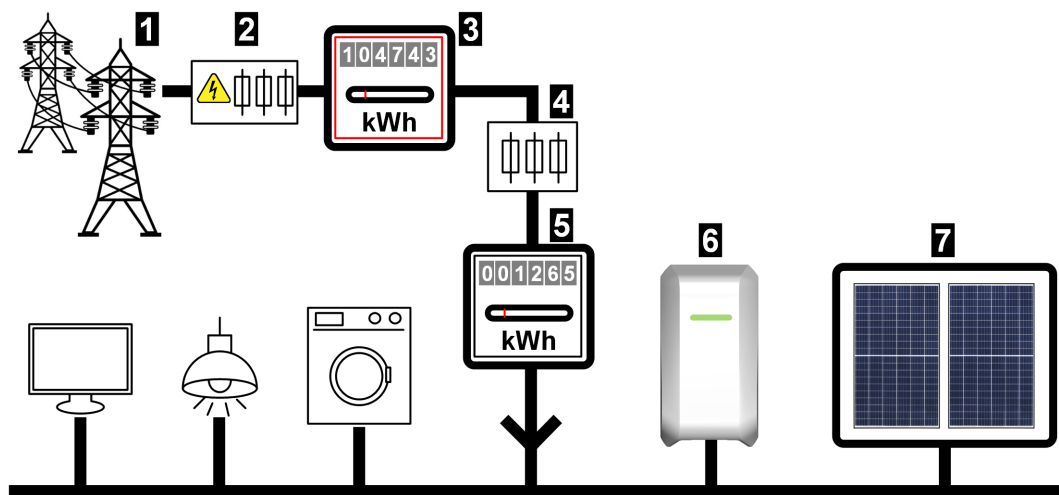
Fig. 14-7: System overview - Integration of an external energy meter
