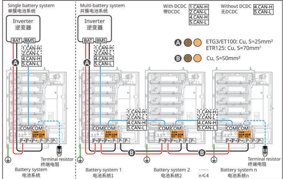
LAN Communication / LAN通信 BATC10ELC0001
