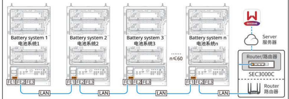
LAN Communication / LAN通信 BATC10ELC0001
