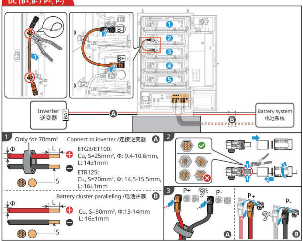
DC (B+, B- / P+, P-) BATC10INT0010
