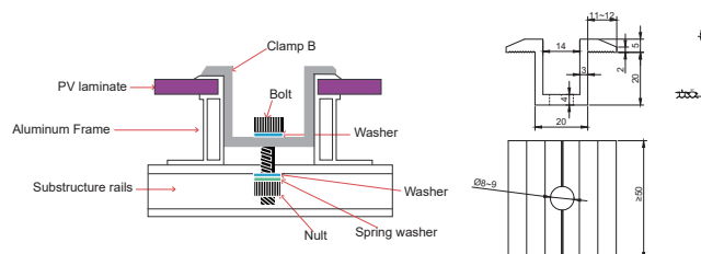
Clamp B The clamp used on the middle module
