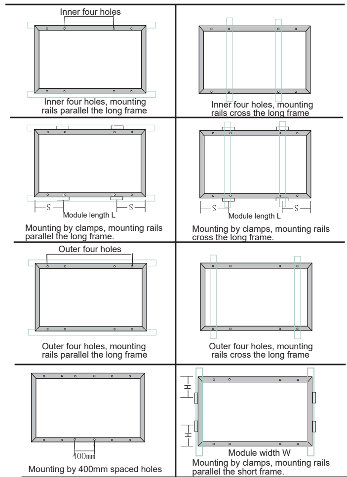
Figure 4 Installation Methods
