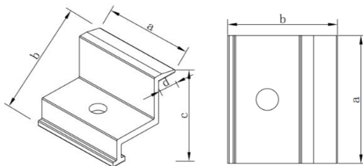
Figure 10. Recommended clamp schematic.
