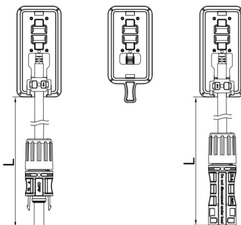
Figure 12. The half-cut cell module/split junction box.
