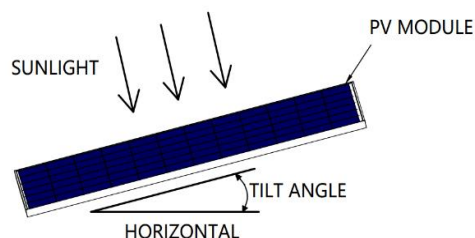
Figure 8 PV module tilt angle.
