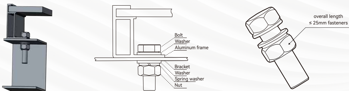
Figure 5 Bolt Installation of Modules
