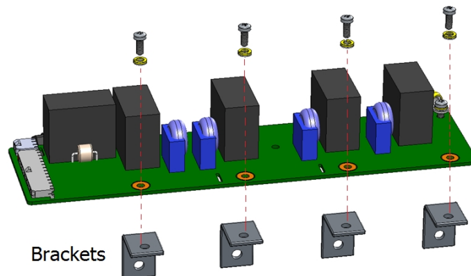
Figure 5: AC SPD Board Brackets Removal
