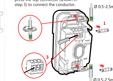
A. Insert cables from top and bottom
