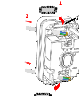
B. Insert cables from behind
