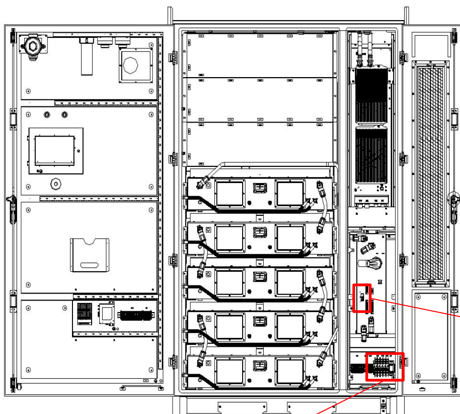
Figure 6.2.2.2 Schematic diagram of the control box
