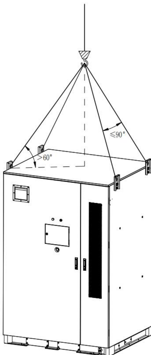
Figure 5.2.3.1 Lifting Schematic
