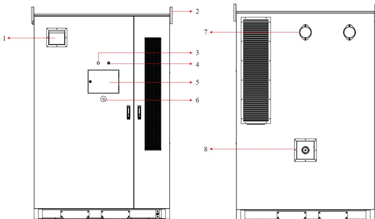
Figure 3.4.2 Main View and Back View
