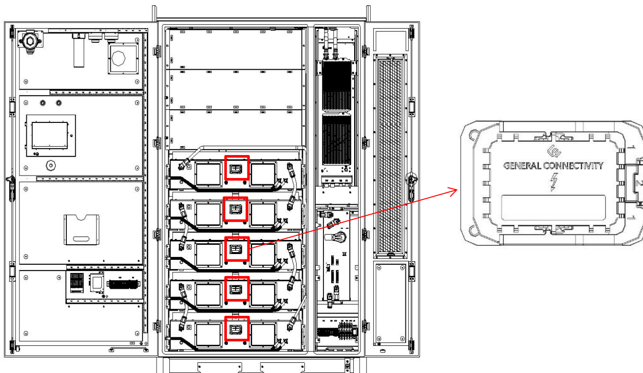
Figure 6.2.2.1 Schematic diagram of the maintenance switch
