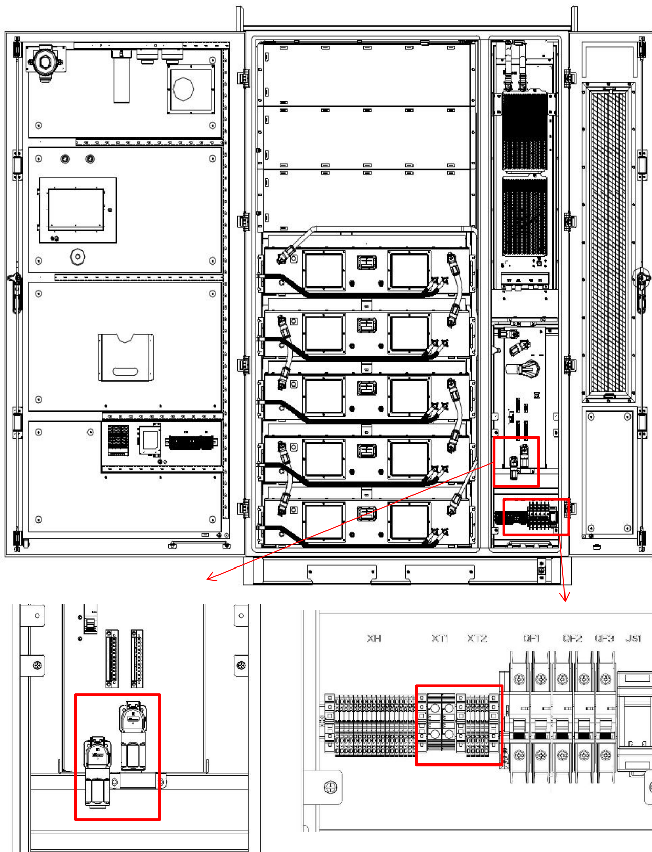
Figure 5.3.4.1 Schematic Diagram of Power Line and Auxiliary Power Supply Line Connection Locations
