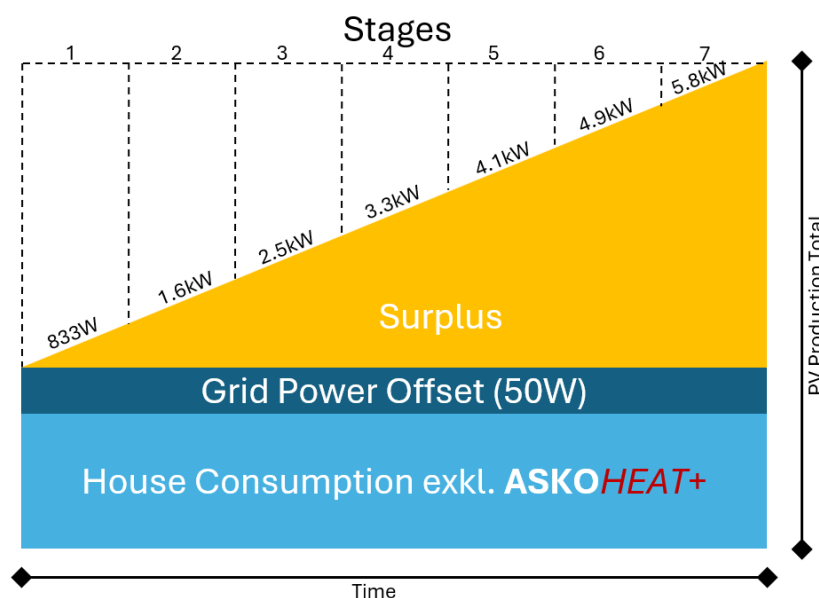
Example of a 7-stage 5.8 kW ASKOHEAT+/+ 2.0
