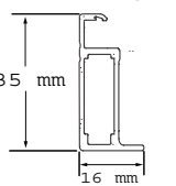
END FRAME PROFILE
