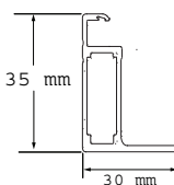
SIDE FRAME PROFILE
